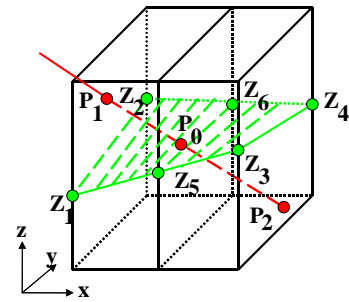
Figure 4. Bilinear surface.
